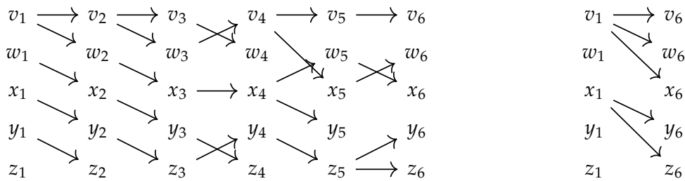
Figure 4: A string of five composable morphisms in the selection category \left[ \begin{array}{c} y^5 \\ y^5 \triangleleft \mathcal{D} \end{array} \right] (left), and their composite (right), obtained by simply following the paths. Each of the arrows shown represents a map in the base category \mathcal{D} . One sees that v_1 and x_1 were the most “fit”, in that they had progeny lasting until the sixth epoch, whereas the others ( w_1, y_1, z_1 ) all went extinct.
